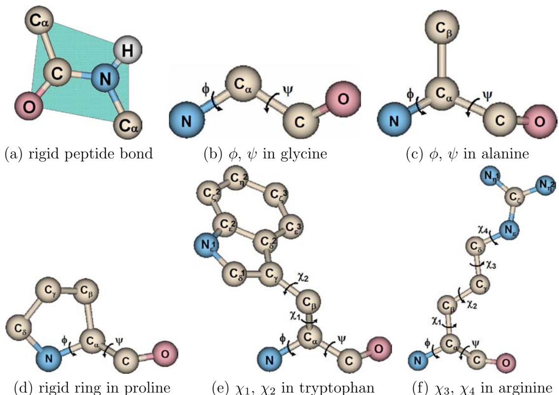
Fig. 2.4: (a) Electron sharing between the carboxyl carbon and the amide nitrogen gives the peptide bond a partial double-bond character and as a consequence its rigidity. (b) and (c) demonstrate the two backbone dihedrals \phi , \psi on two amino acids, glycine, and alanine. (d) No side-chain dihedrals for the rigid ring in Proline (e) Tryptophan contains 2 side-chain dihedrals (f) Arginine has the highest number of side-chain dihedrals, 4. Figures are generated with MOLMOL [KBW96].
