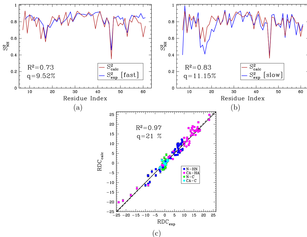
Fig. 4.3: Comparison of NMR data with thermodynamics data obtained by PEM for protein G. (a) Comparison of PEM-obtained S^2 backbone (amide) order parameters ( S^2_{calc} ) with fast S^2_{NH} data obtained from NMR relaxation measurements ( S^2_{exp} ). (b) Comparison of PEM-obtained S^2 backbone (amide) order parameters ( S^2_{calc} ) with slow S^2_{NH} data obtained from NMR relaxation measurements ( S^2_{exp} ). (c) Comparison of residual dipolar coupling (RDC) parameters obtained by PEM ( RDC_{calc} , on the y-axis), and obtained from NMR relaxation experiments ( RDC_{exp} , on the x-axis). Results for different bond types are shown in different colors. (a)-(c) The dashed black line indicates the linear least squares regression fit on the two sets of data, while the continuous line represents the identity line.
