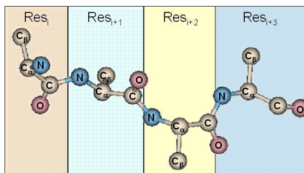
Fig. 2.1: (a) Polypeptide chain with four amino acids. C_\beta is the only side-chain atom shown. Figure is generated with MOLMOL [KBW96].
