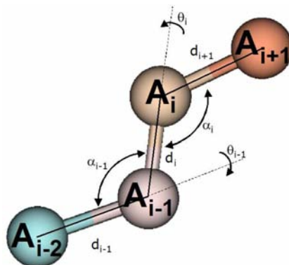
Fig. 2.5: A protein can be modeled as an articulated mechanism, where d_i is the length of the bond between atoms A_{i-1} and A_i , \alpha_{i-1} the bond angle between A_{i-2} , A_{i-1} , and A_i , \theta_{i-1} the \psi dihedral, and \theta_i the \phi dihedral. Figure is generated with MOLMOL [KBW96].
