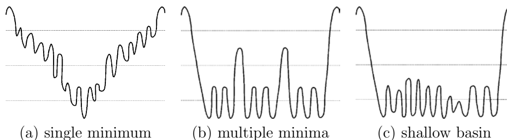
Fig. 2.6: (a) The native structure is a strong stability point, reflected in the single global minimum. (b) There are multiple global minima in the energy landscape. (c) The native structure is not a strong stability point, resulting in a shallow basin.
