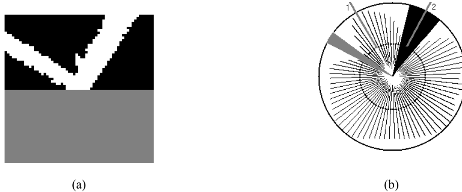
Figure 3: (a) A sample 2D grid-based local map computed from laser readings. White color corresponds to free space, black color corresponds to obstacles and gray color corresponds to lack of information. (b) The vector histogram created from Fig 5(a). Light gray sector defines a non-safe (narrow) space and the dark gray sector defines a safe (wide) space. Although the target direction is along line 1, PYTHEAS will follow the direction along line 2.
