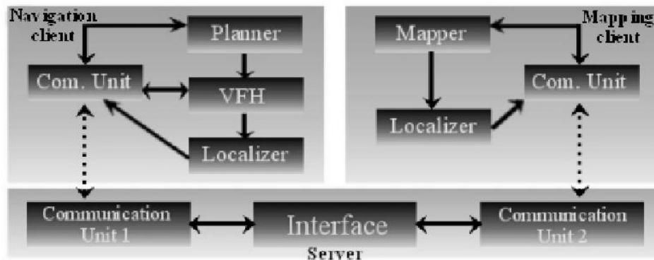
Figure 4: Overview of the integration architecture.
