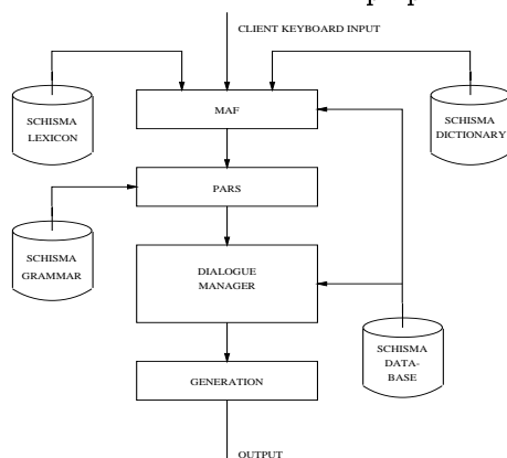
Figure 1: Global architecture of SCHISMA
